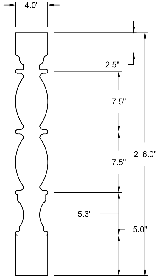
Spindle Profile view
