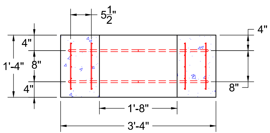
Section B-B
